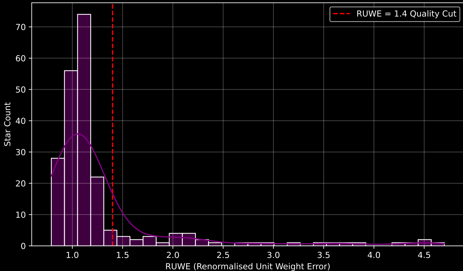
GALAH DR4 Field [7236] RUWE Distribution (n= 218)
