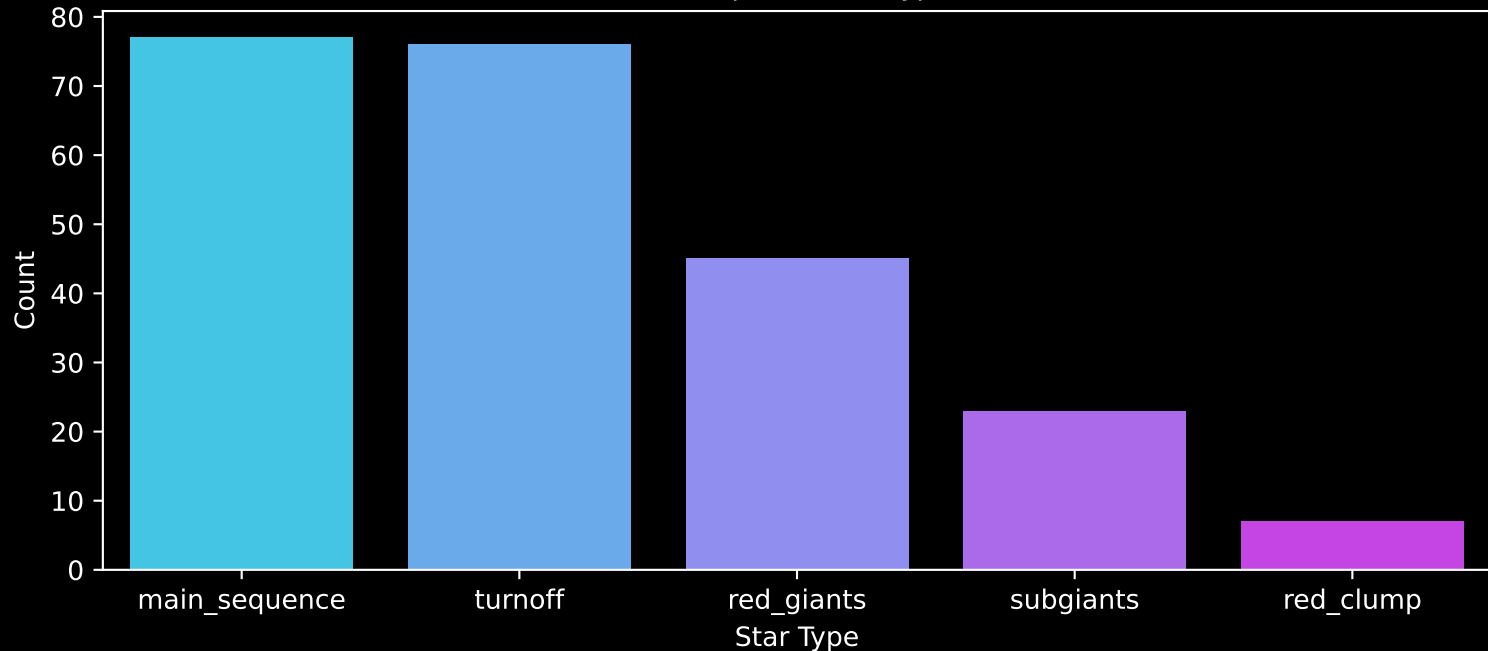
GALAH DR4 Field: [7236] Count plot of Star Type
