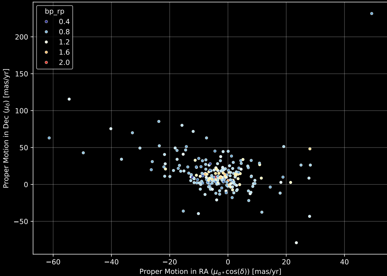
GALAH DR4 Field: [7236] Proper Motion Diagram (n= 228)
